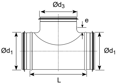
T piece (pressed)
