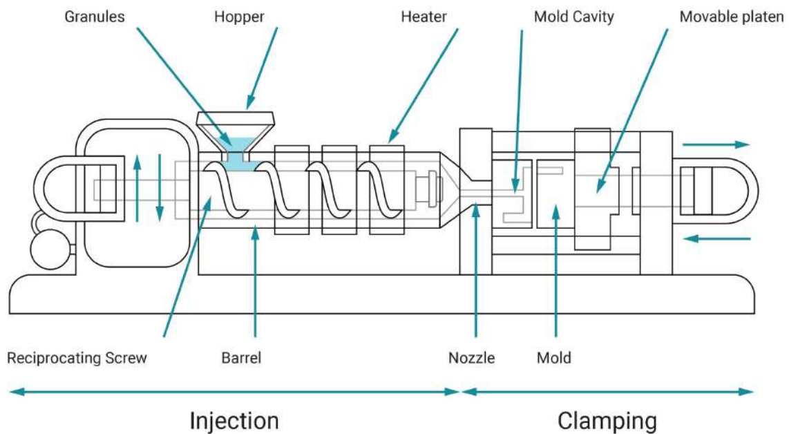
Injection Molding Machine
