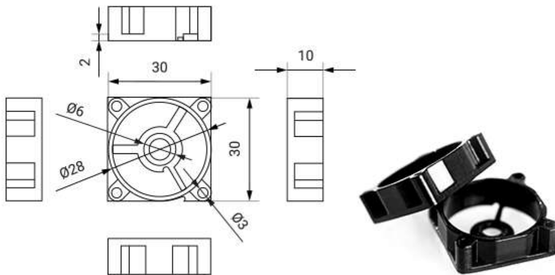
A computer fan cover design used in the study
