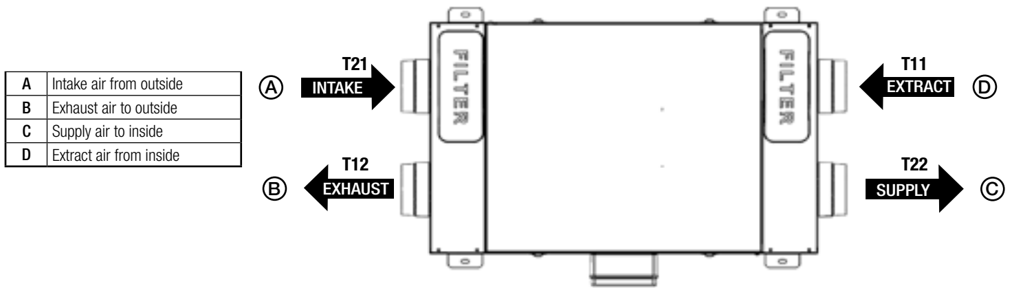
Fig. 7.a Temperature probes
