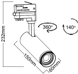
4 CABLES 3-PHASE
