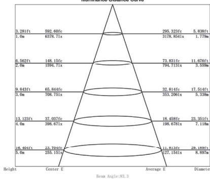
Illuminance-Distance Curve
