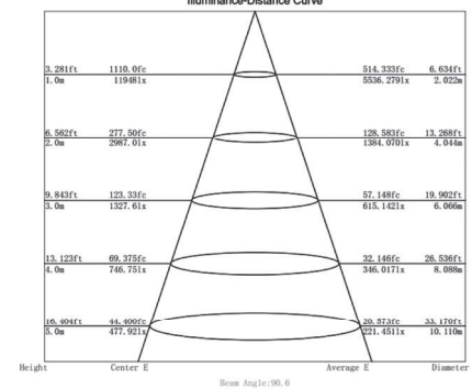
Illuminance-Distance Curve
