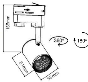
4 CABLES 3-PHASE
