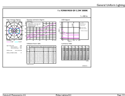
CorePro LEDcapsule ND 3.2-40W G9 830
