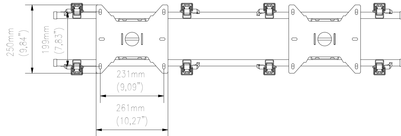
TOP VIEW
