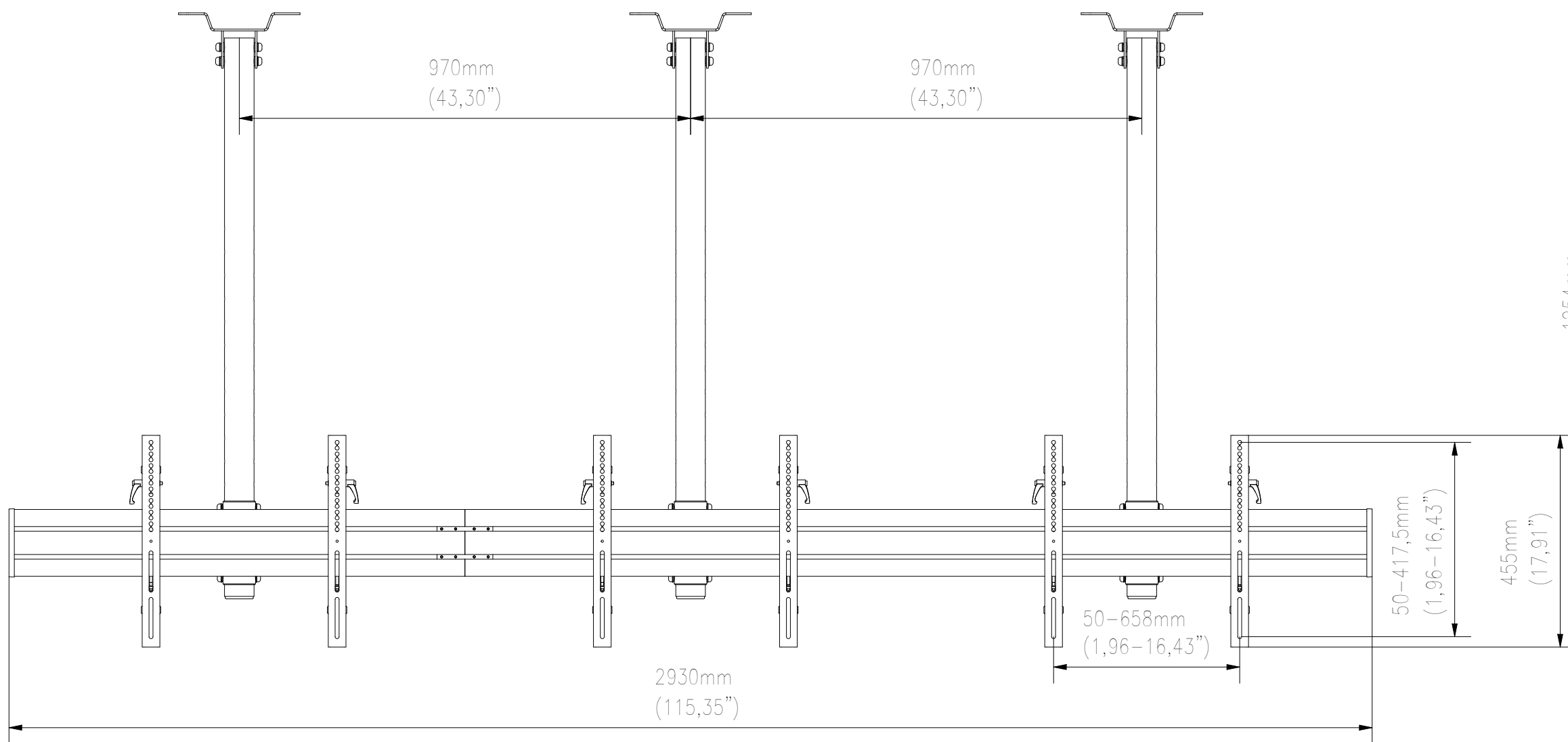
FRONT VIEW
