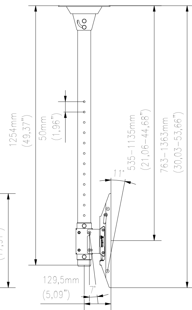
SIDE VIEW
