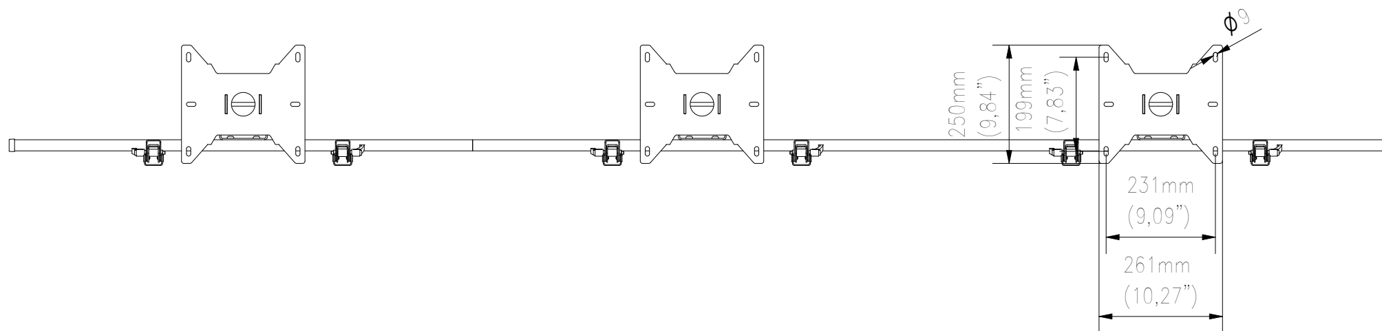
TOP VIEW
