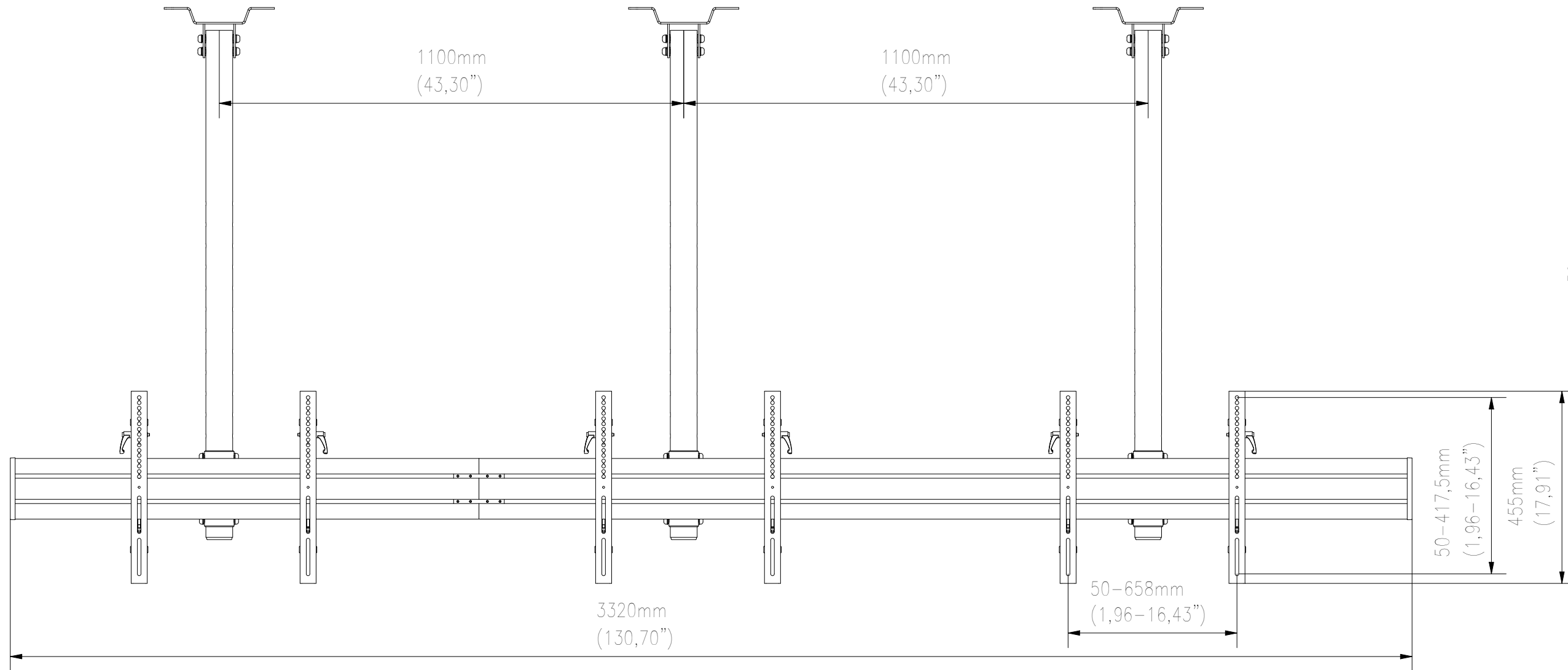
FRONT VIEW
