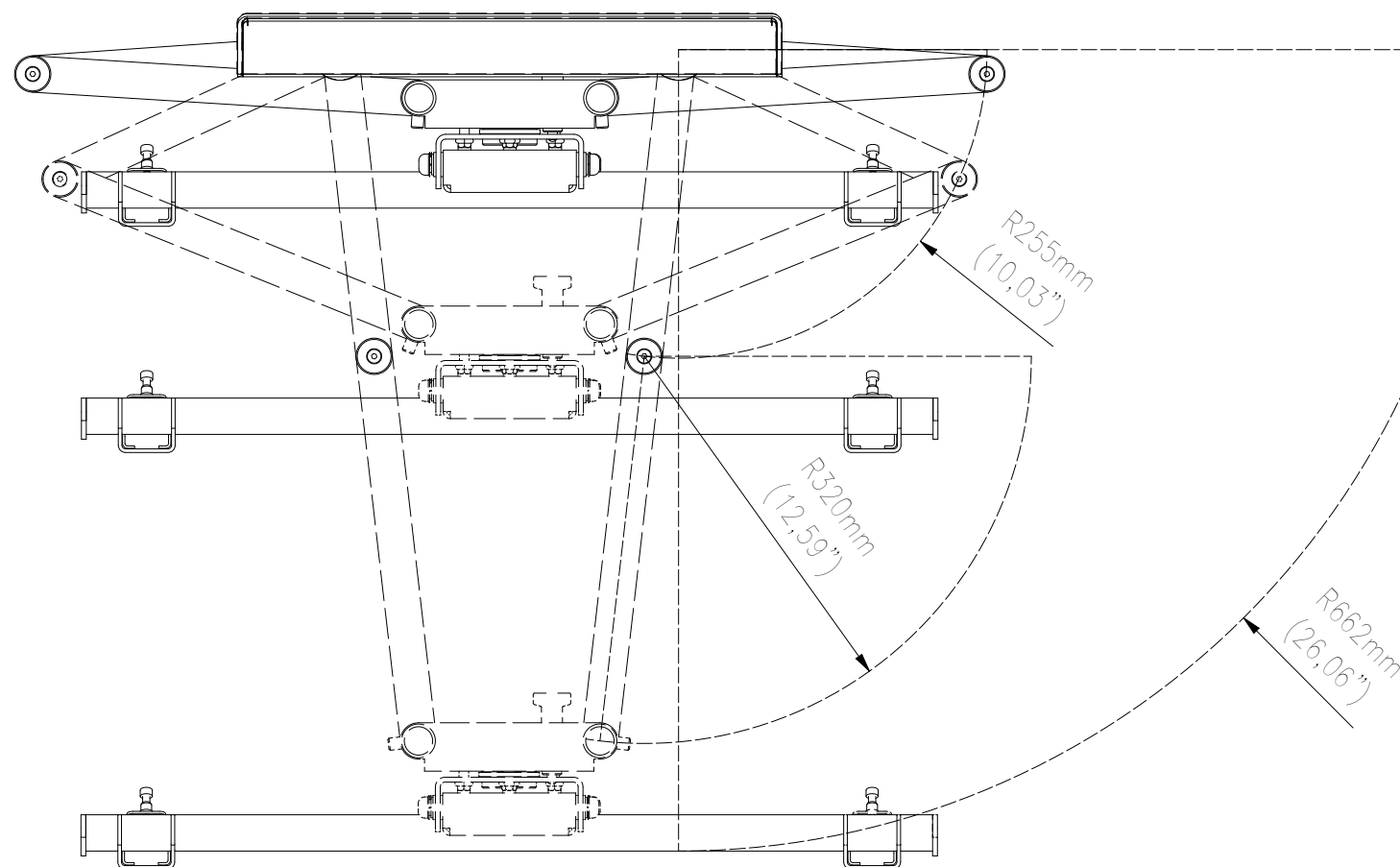
TOP VIEW
