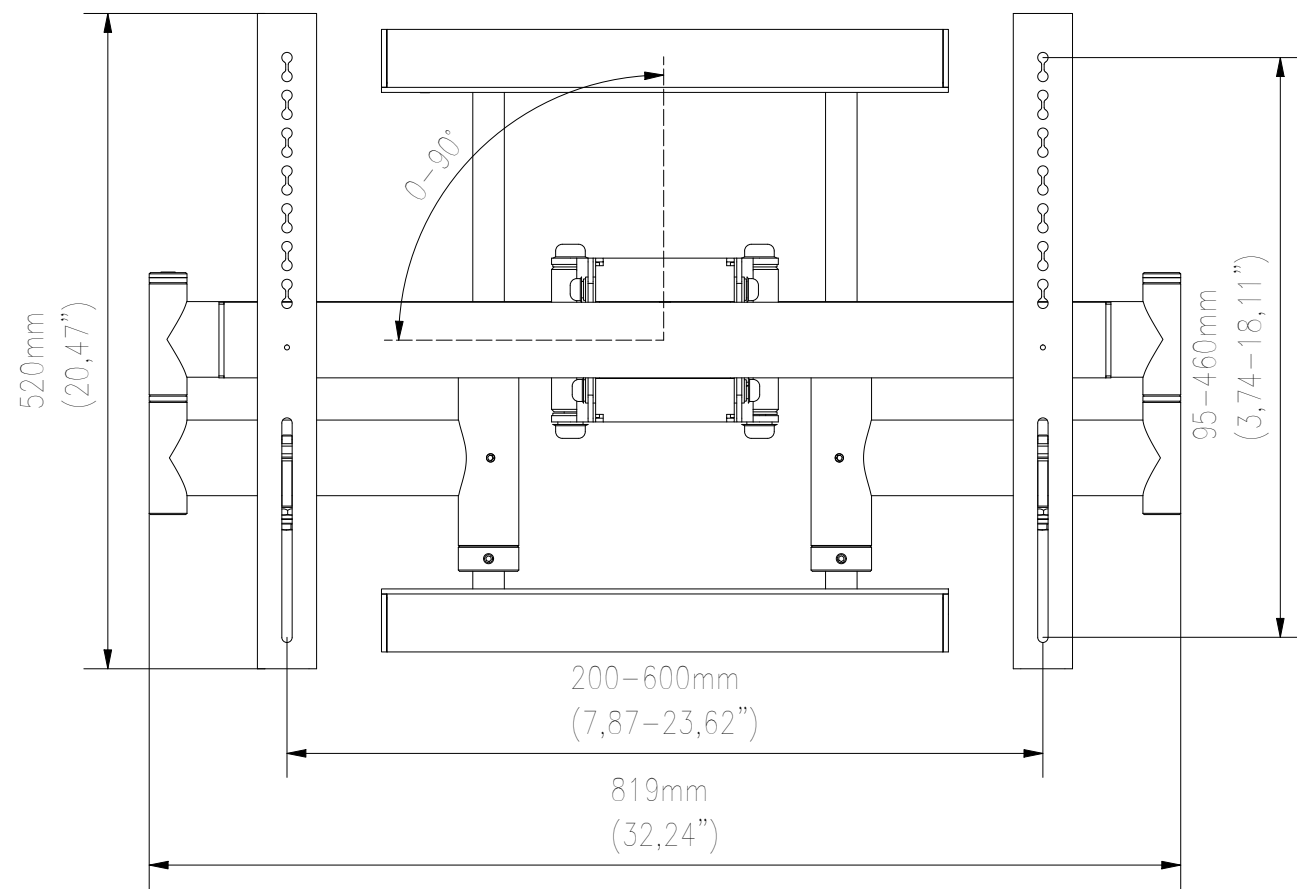
TOP VIEW
