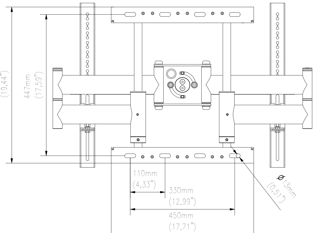
REAR VIEW
