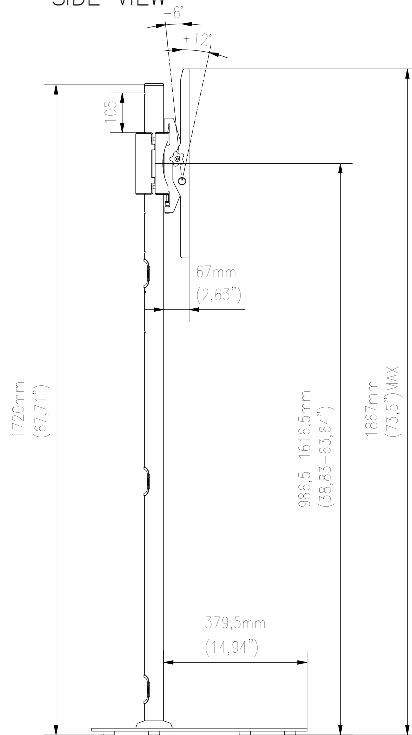
SIDE VIEW
