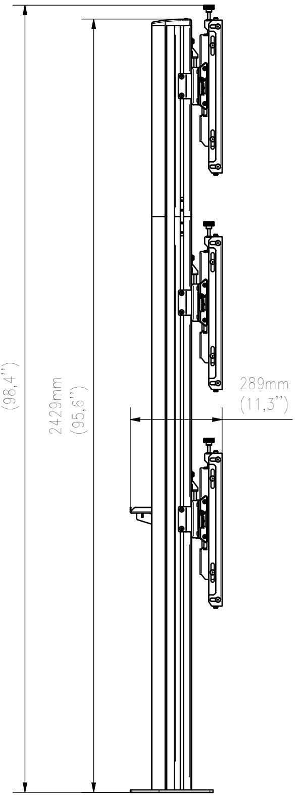
SIDE VIEW
