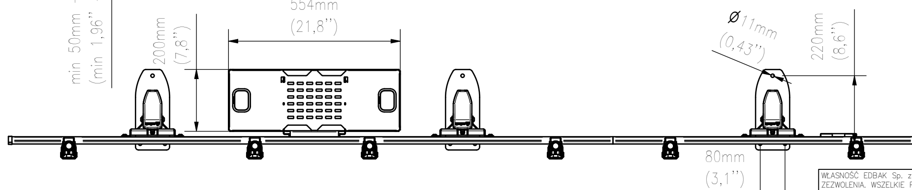
TOP VIEW
