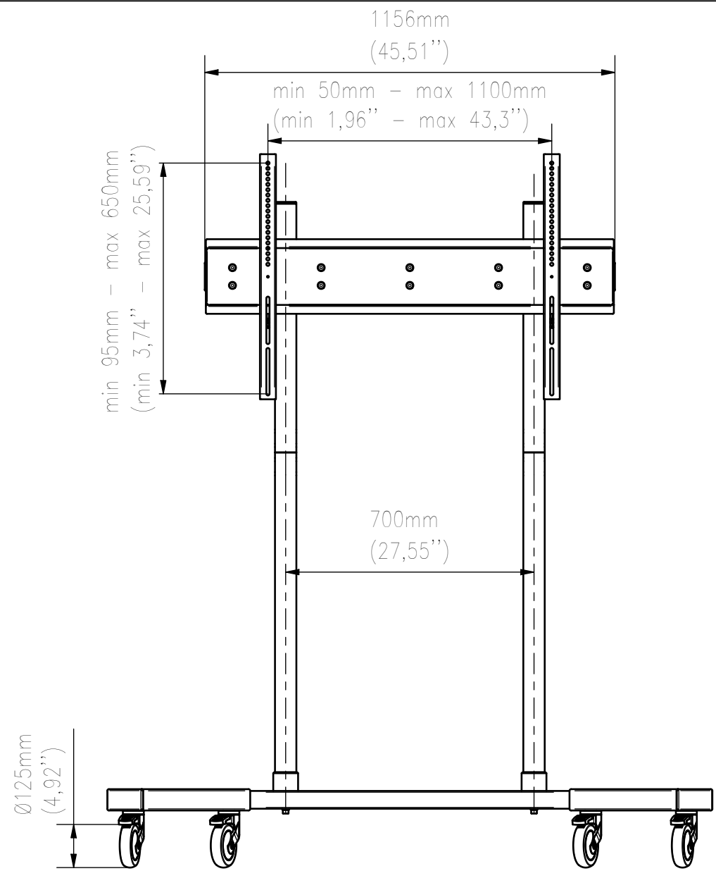
FRONT VIEW
