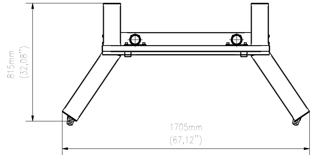
TOP VIEW
