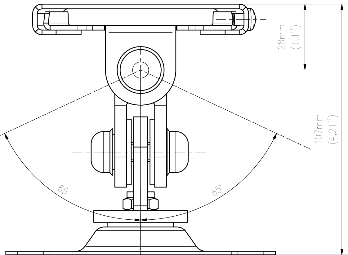
TOP VIEW
