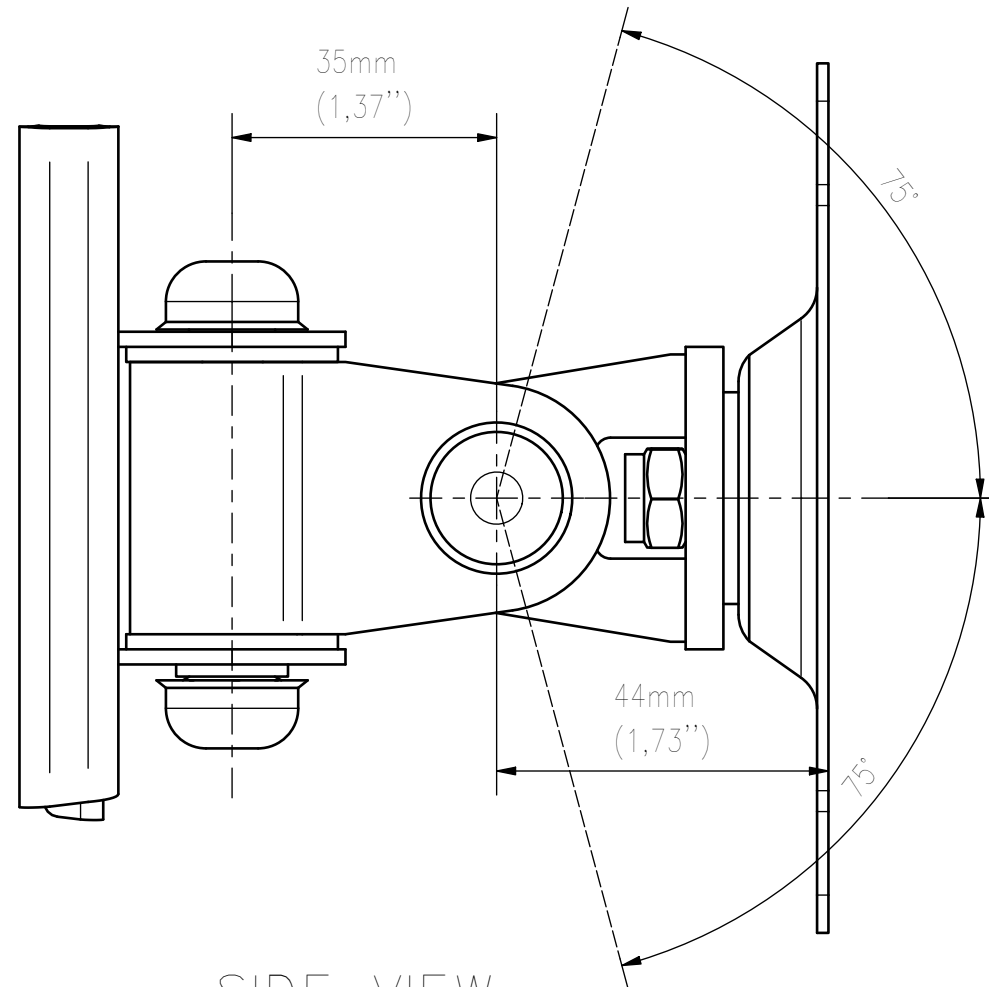
SIDE VIEW
