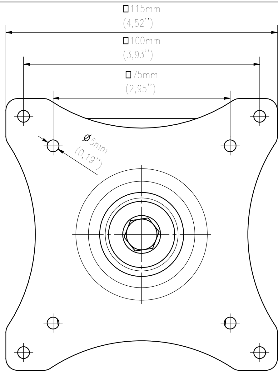
FRONT VIEW
