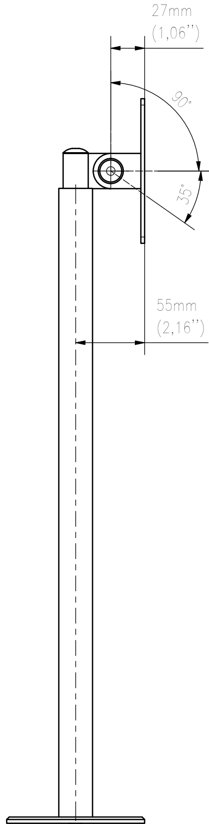
SIDE VIEW
