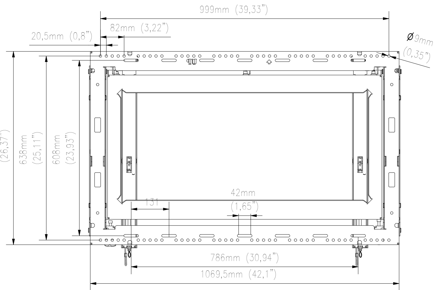
REAR VIEW
