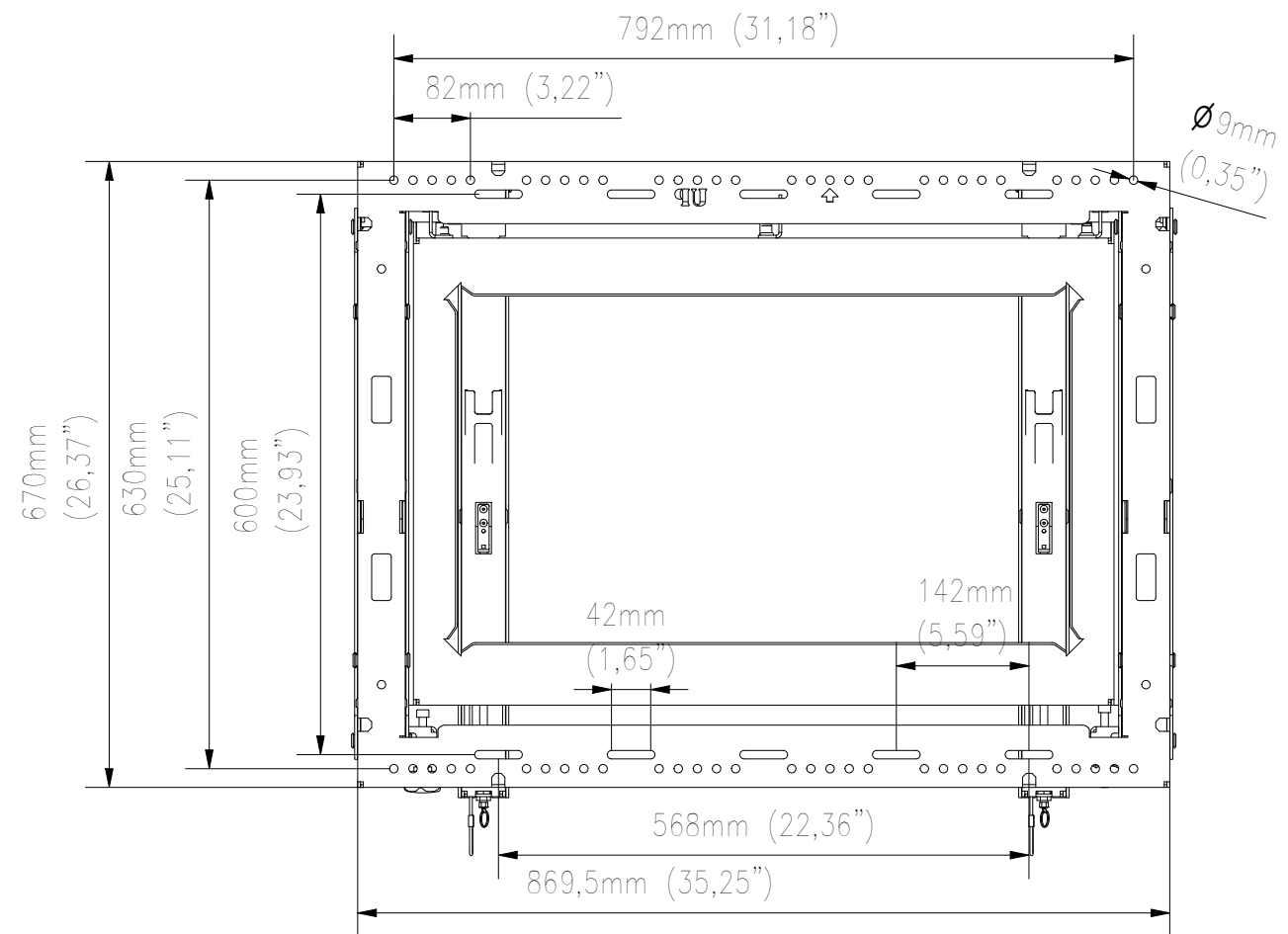
REAR VIEW
