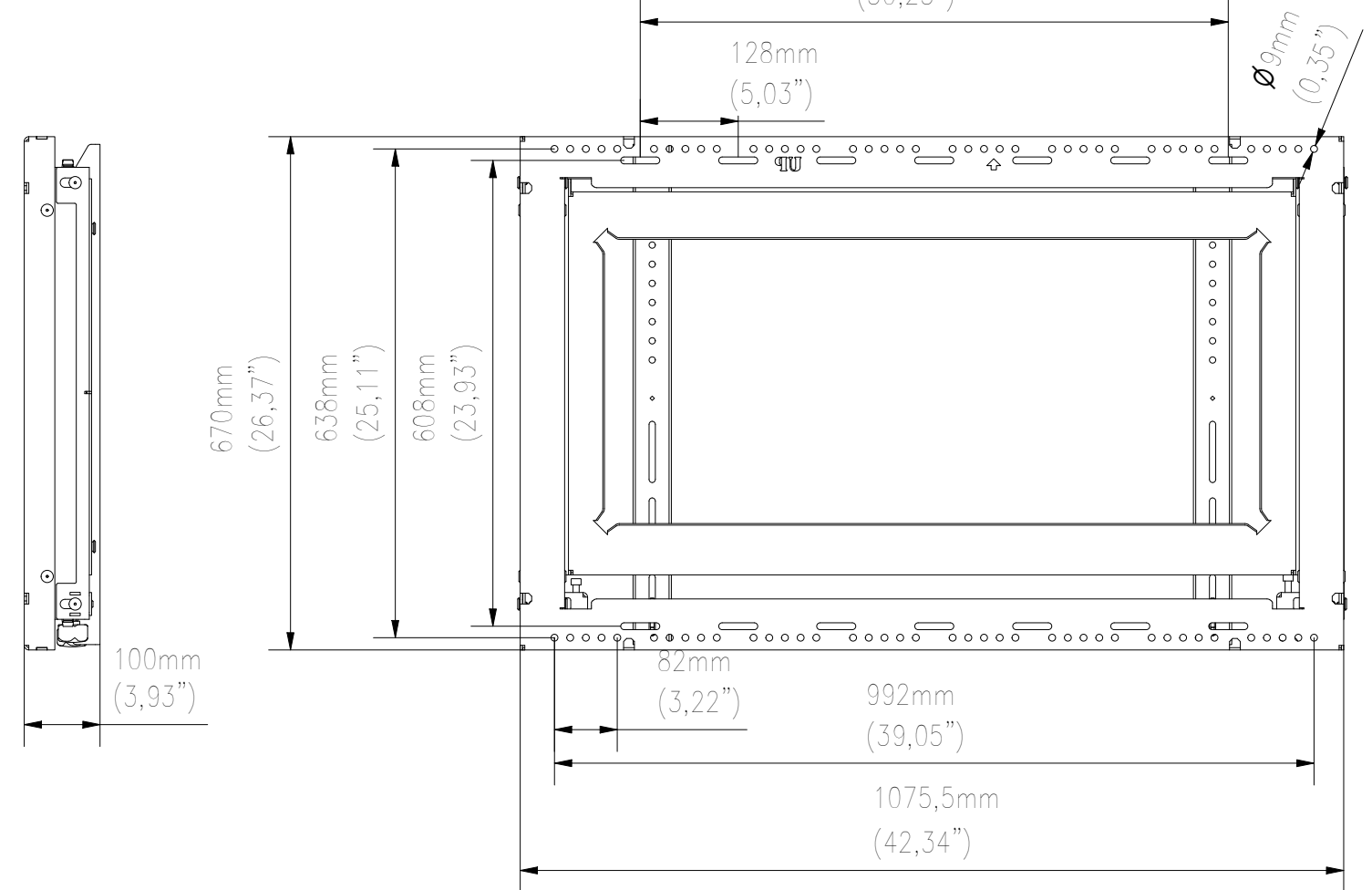
REAR VIEW 768mm (30,23")
