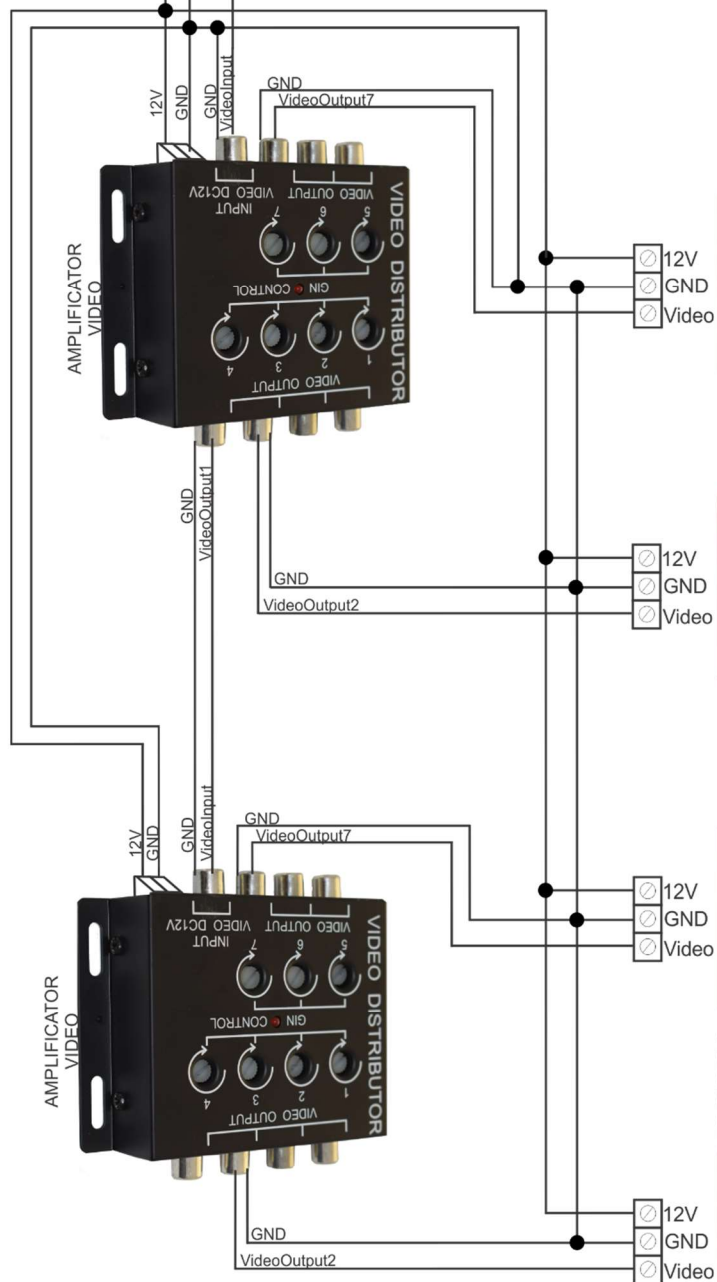
INTERFON DE SCARA ISCP-01N-50 VIDEO
